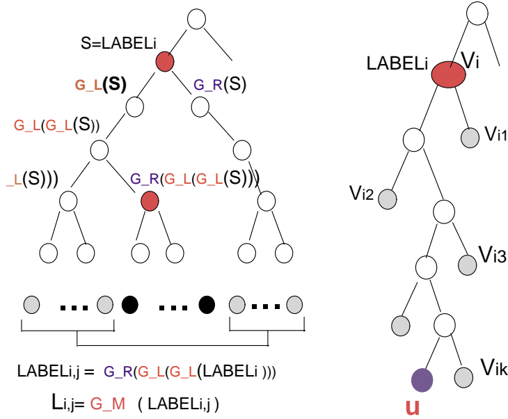
Figure 3: Key Assignment in the Subset Difference Method. Left : generation of LABEL_{i,j} and the key L_{i,j} . Right : leaf u receives the labels of v_{i_1}, \dots, v_{i_k} that are induced by the label LABEL_i of v_i .
